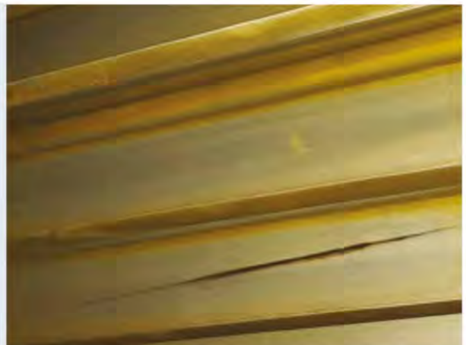
Figure 5 Fretting corrosion across the tooth flank
