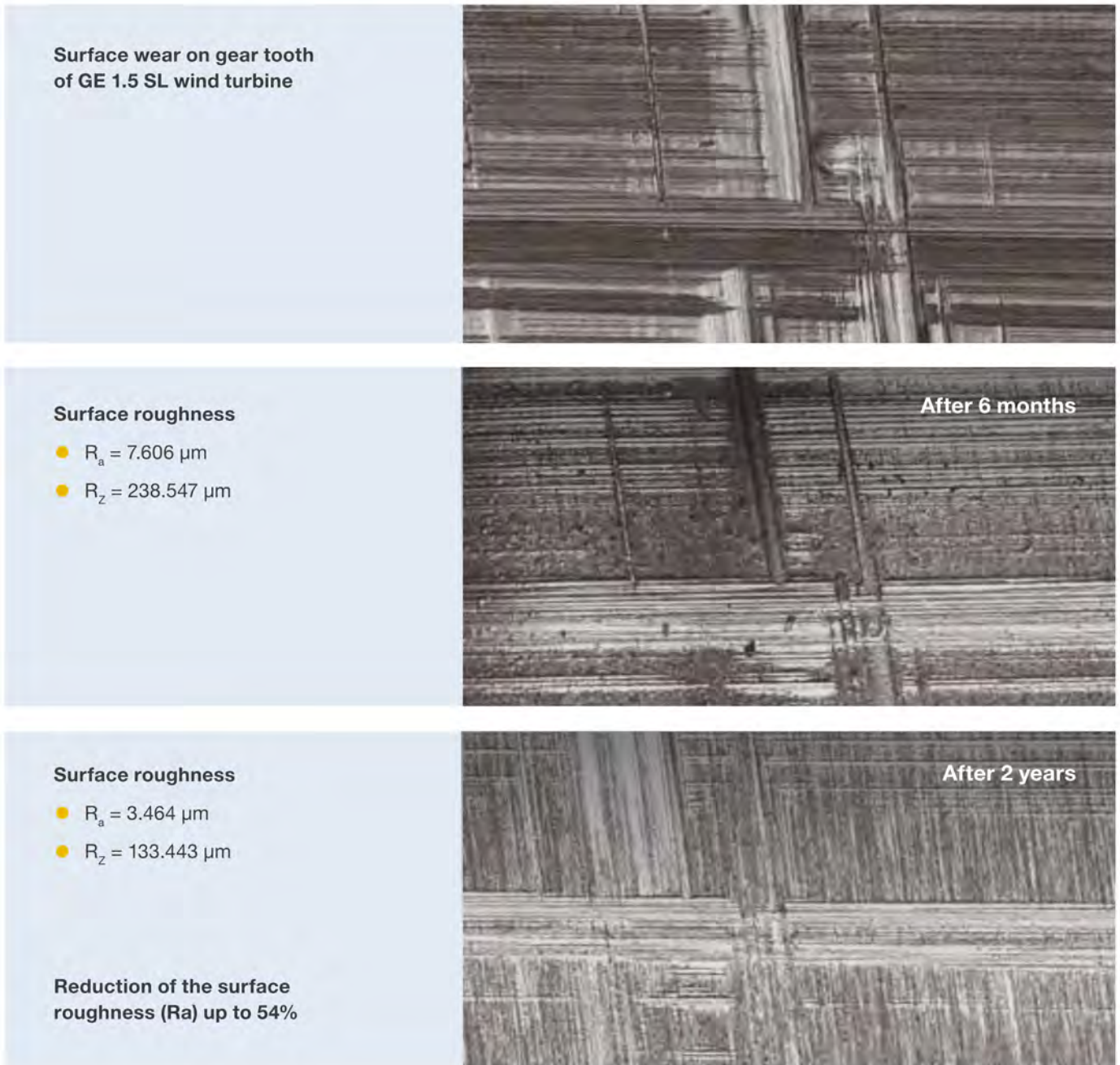
Figure 22 Surface roughness evaluations before and after the application of REWITEC
